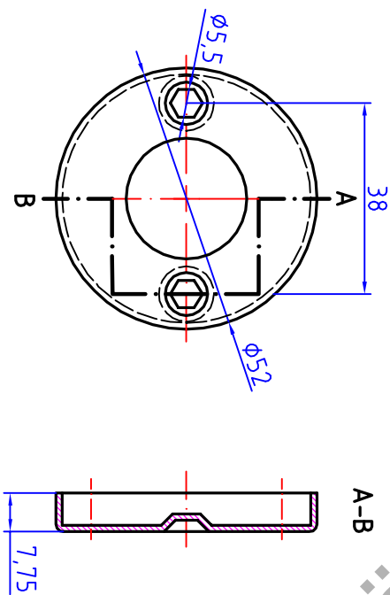
Innenteil (inside part)
